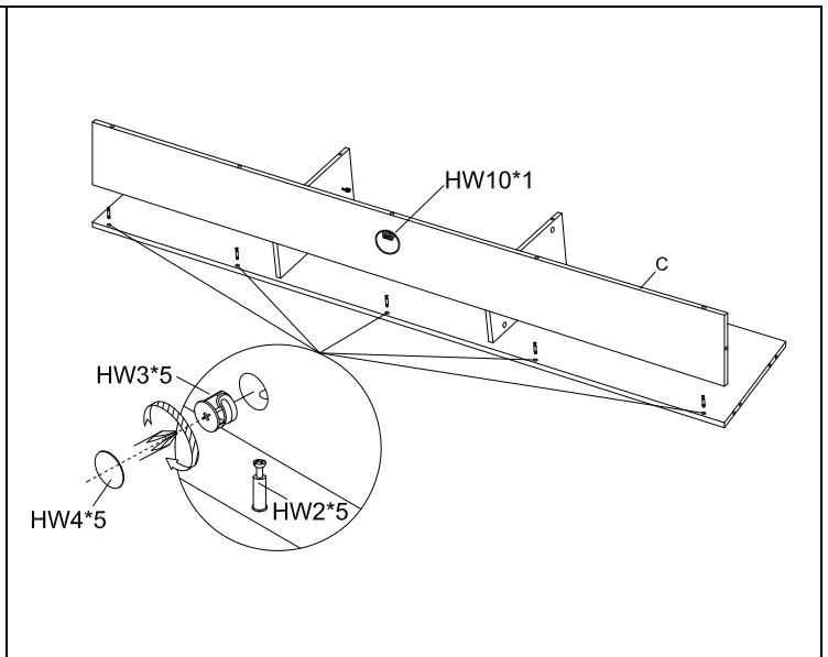
STEP2 assemble the back panel
