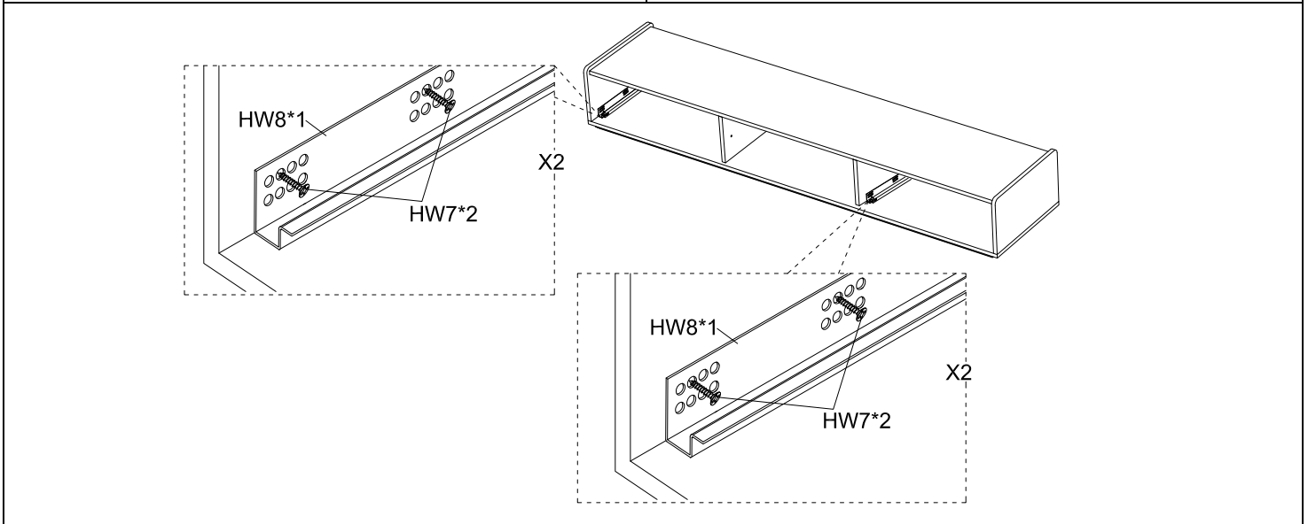
STEP5 assemble the slide runner
