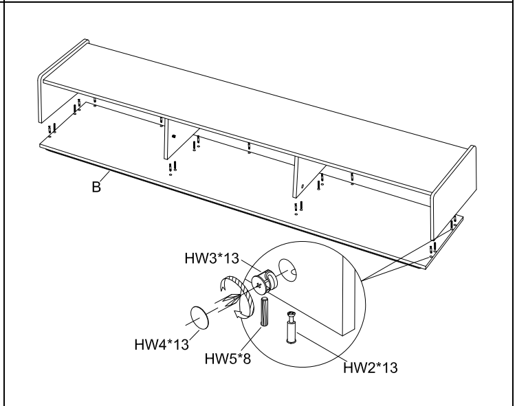
STEP4 assemble the back panel
