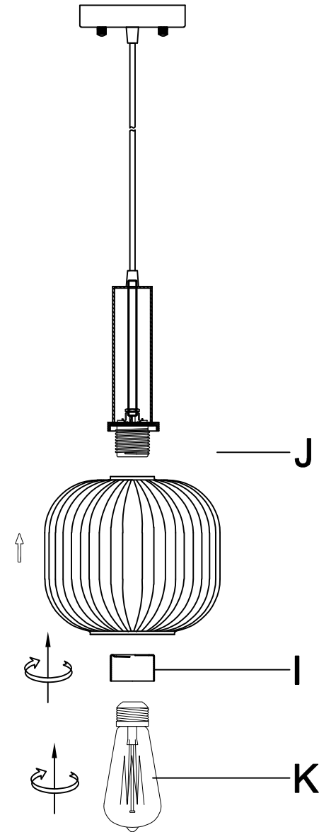
Step 5: Fix the glass (J) on the lamp holder with the lamp shade (I) .and then fix the bulb (K) into the lamp holder
