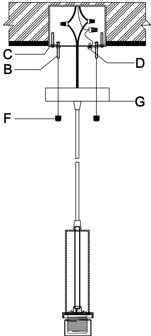
Step 4: Attach the canopy (G) to the Mounting Plate (C), and fix it by turning the canopy nut (F) anti clockwise
