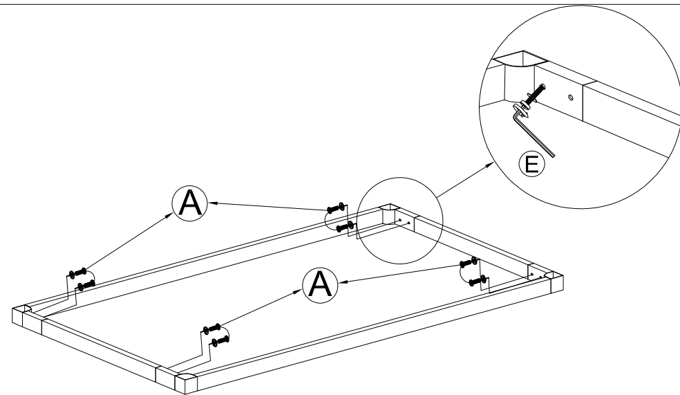
STEP 2: Connect The Part from STEP 1, tighten Bolt (A), Flat Washer (D) with Allen key (E).
