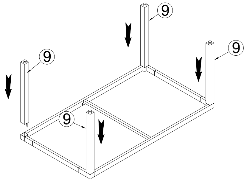
STEP 4: Connect The Part from STEP 3 and Table Leg (9).
