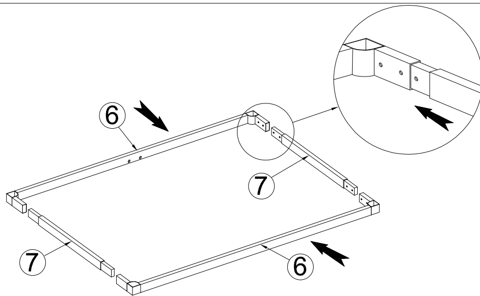
STEP 1: Connect Long Table Top Frame (6) and Short Table Top Frame (7).
