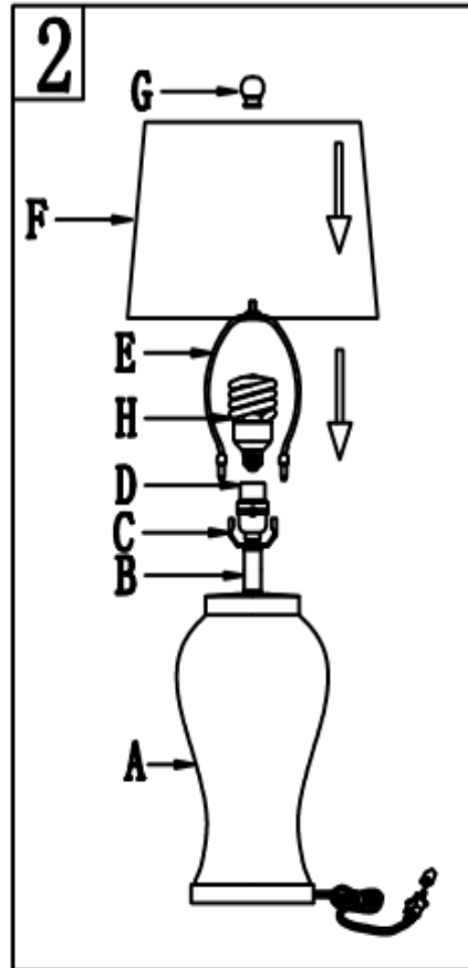
Step 2 Insert the Harp (E) into the Saddle (C). Put the shade (F) on the Harp (E), then tighten the Finial (G) into the Harp (E). Insert the bulb (H) into the socket (D).
