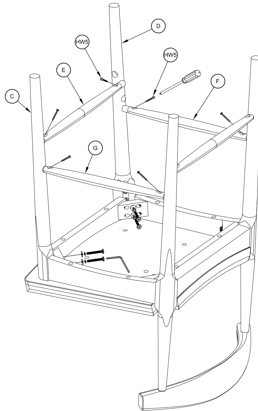
STEP 2: Attach the front legs, front rail and side rails as illustrated in picture. Make sure to apply all the bolts into the holes properly before tightening.
