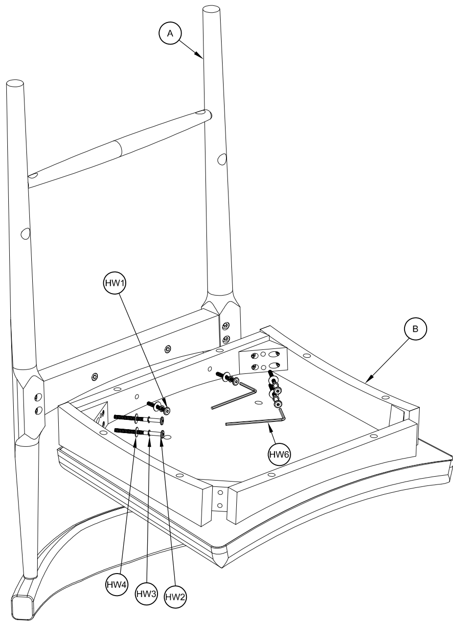
STEP 1: Attach the seat to the chair back. Make sure to apply all the bolts into the holes properly before tightening.
